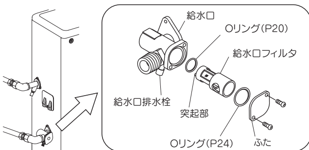
(M) (MS) タイプ
