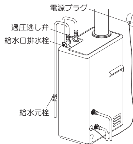
(F)(FK)(FF)(FFK)タイプ
